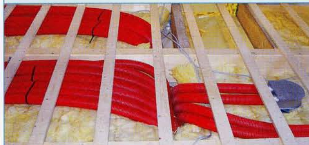
Between joists
