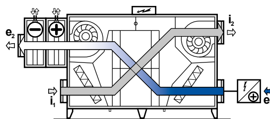
3. Equal pressure ventilation with heating / cooling / or preheating
