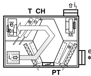
Recirculation mode with optional heating and cooling
