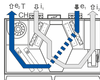
Bypass mode (without heat recovery)
