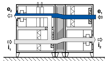
Combined mode (heat recovery mode with recirculation)
