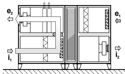
Recirculation mode with heating and cooling
