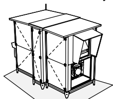
configuration 60/x - door-side view (up to 4 configurations in total)
