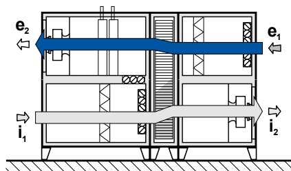
Heat recovery mode with re-heating and cooling
