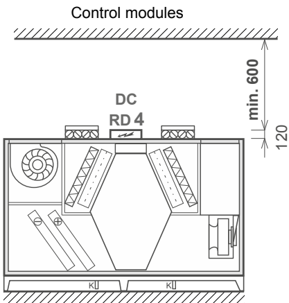
MANIPULATION SPACE FOR UNIT ACCESSORIES
