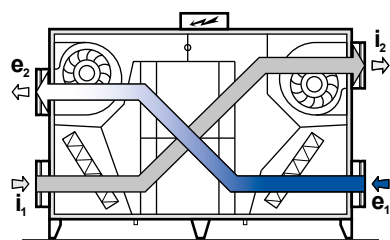
1. Equal pressure ventilation with heat recovery
