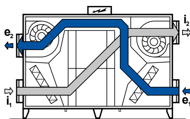
2. Equal pressure ventilation without heat recovery (through by-pass)
