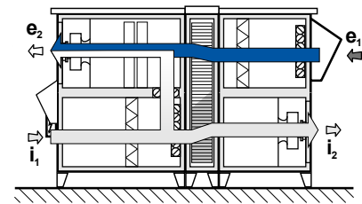
Combined mode (heat recovery mode with recirculation)
